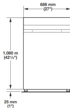
Vista frontal
